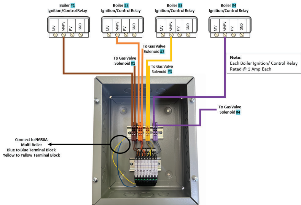
Electrical Connection Diagram
