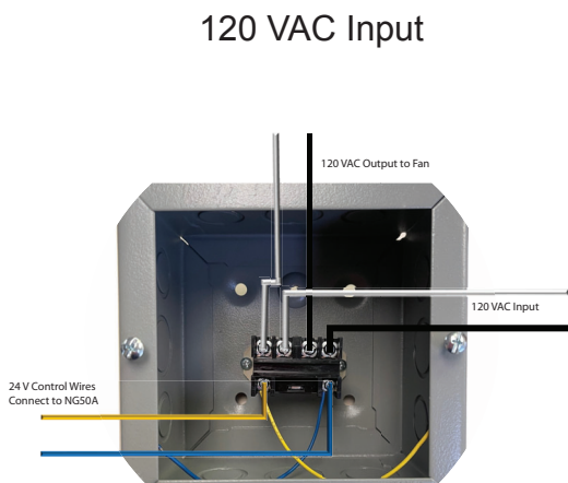
Electrical Connection Diagram
