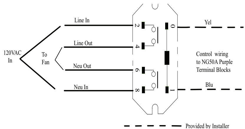
Electrical Schematic
