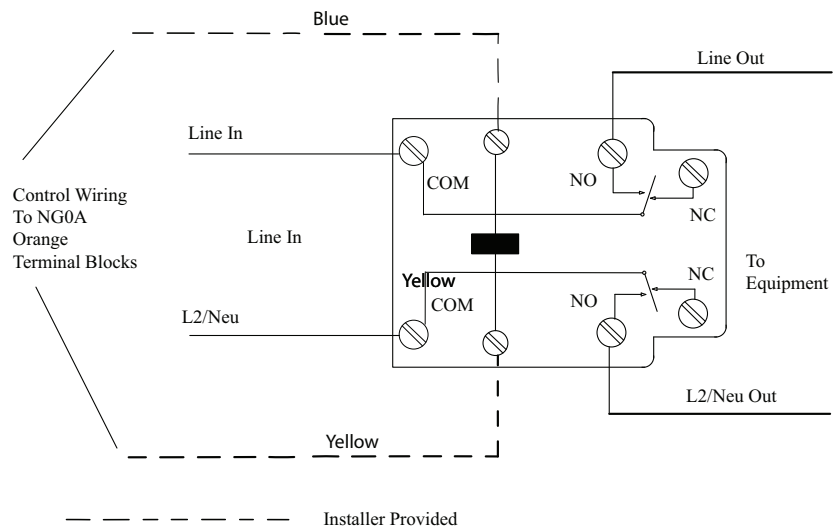
Electrical Schematic
